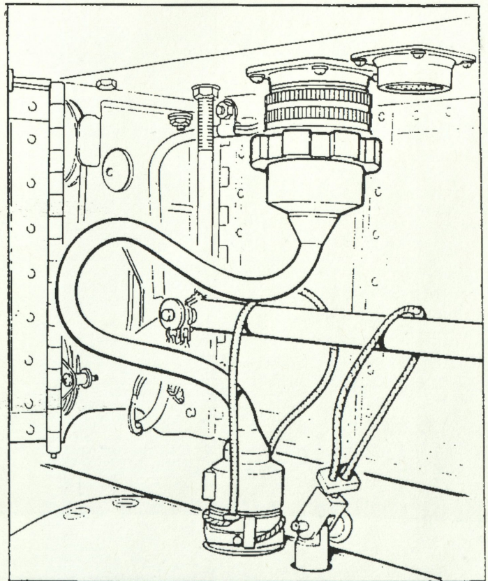
Figure 33. B61-6,8 Aircraft Interface
